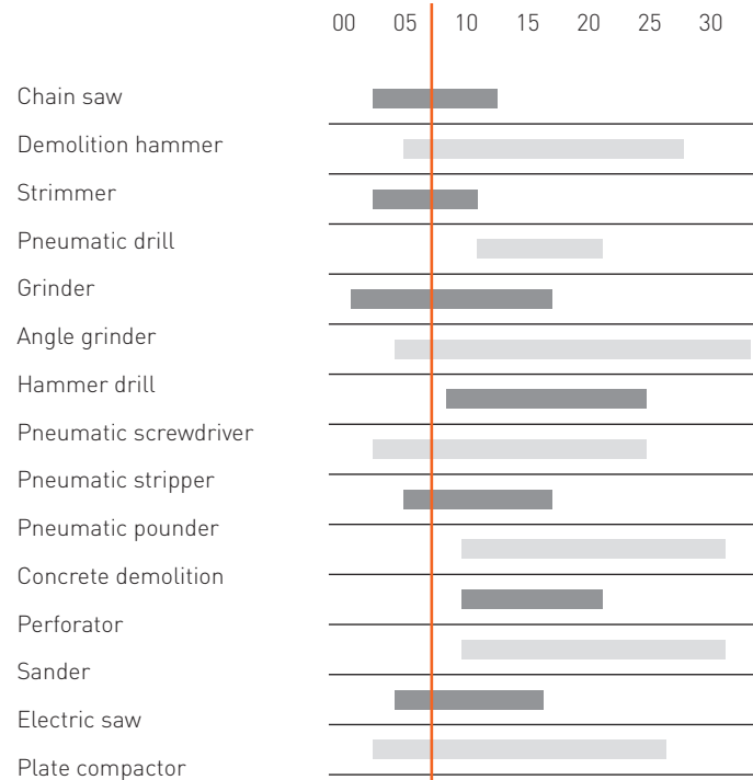
ESTIMATION OF RISKS and wrist Comparison of vibration levels of common and authorised tools in the European Market.
